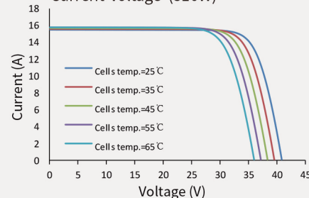
Current-Voltage (510W)
